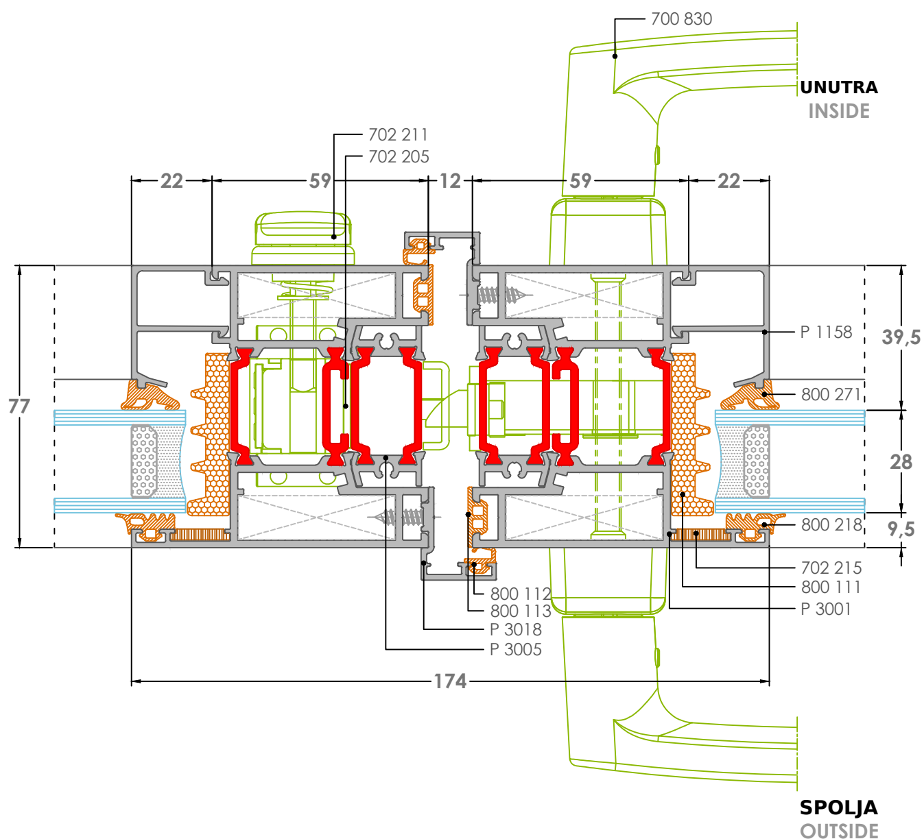
4K-3 DETALJ-Detail
