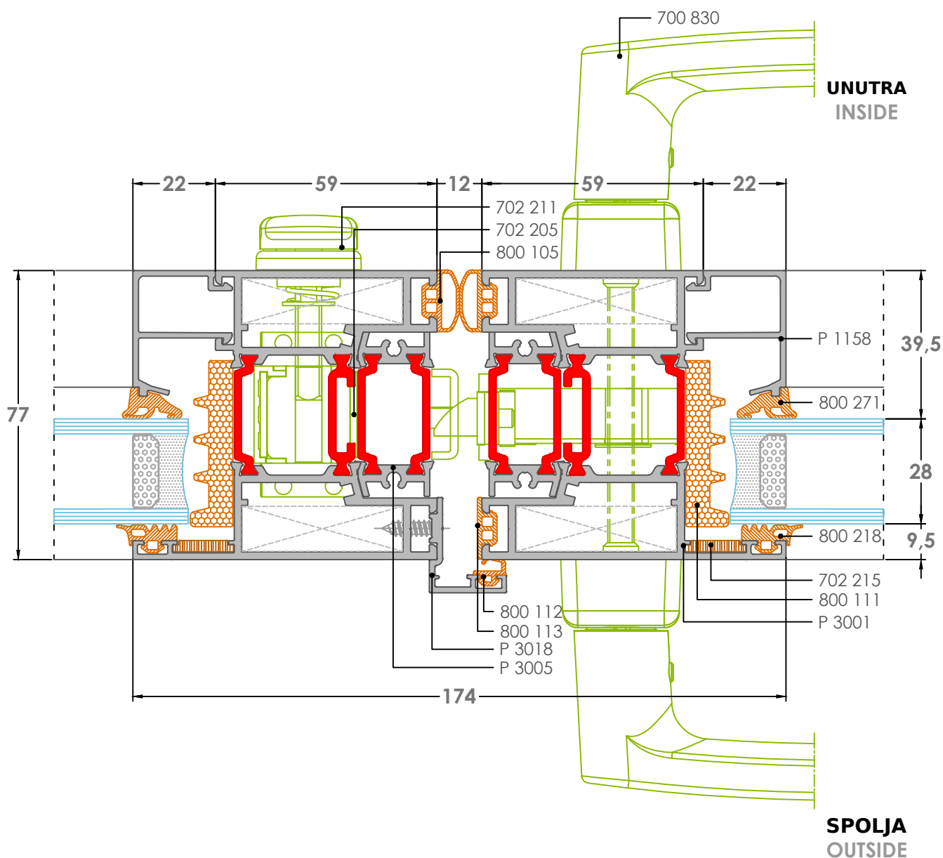
4K-2 DETALJ-Detail
