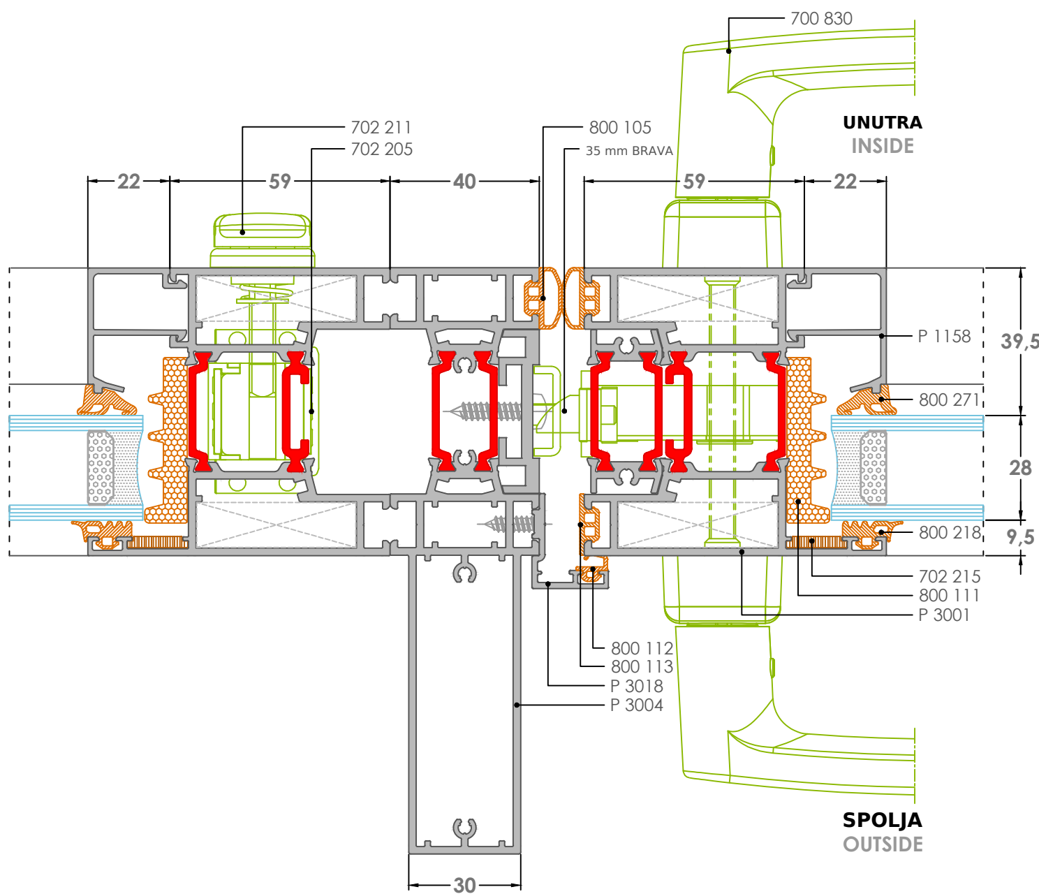
4K-4 DETALJ-Detail
