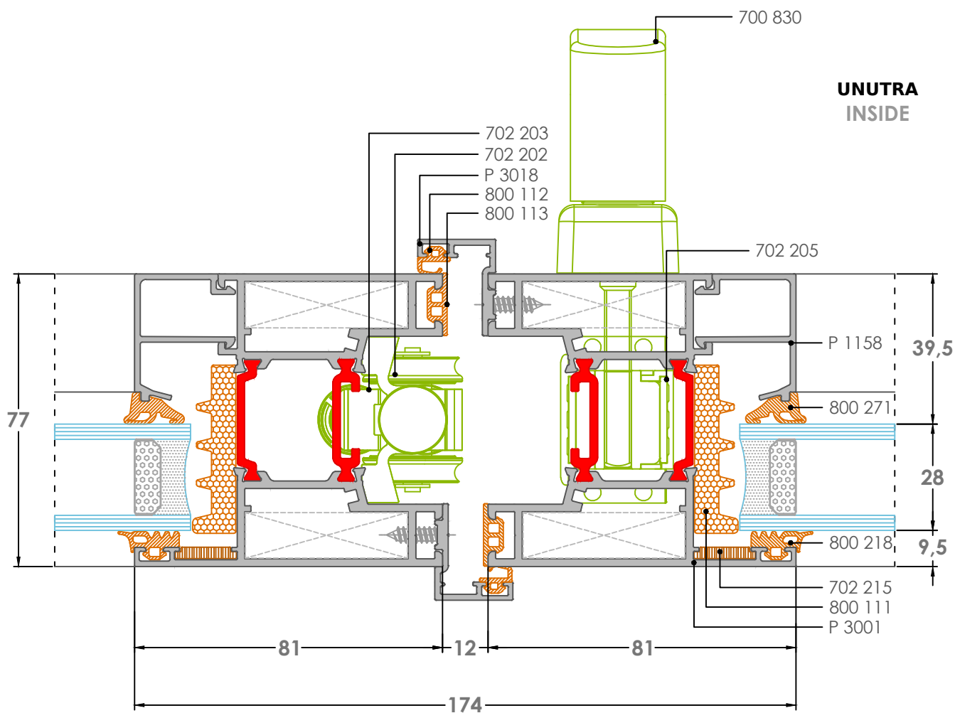
12K DETALJ-Detail
