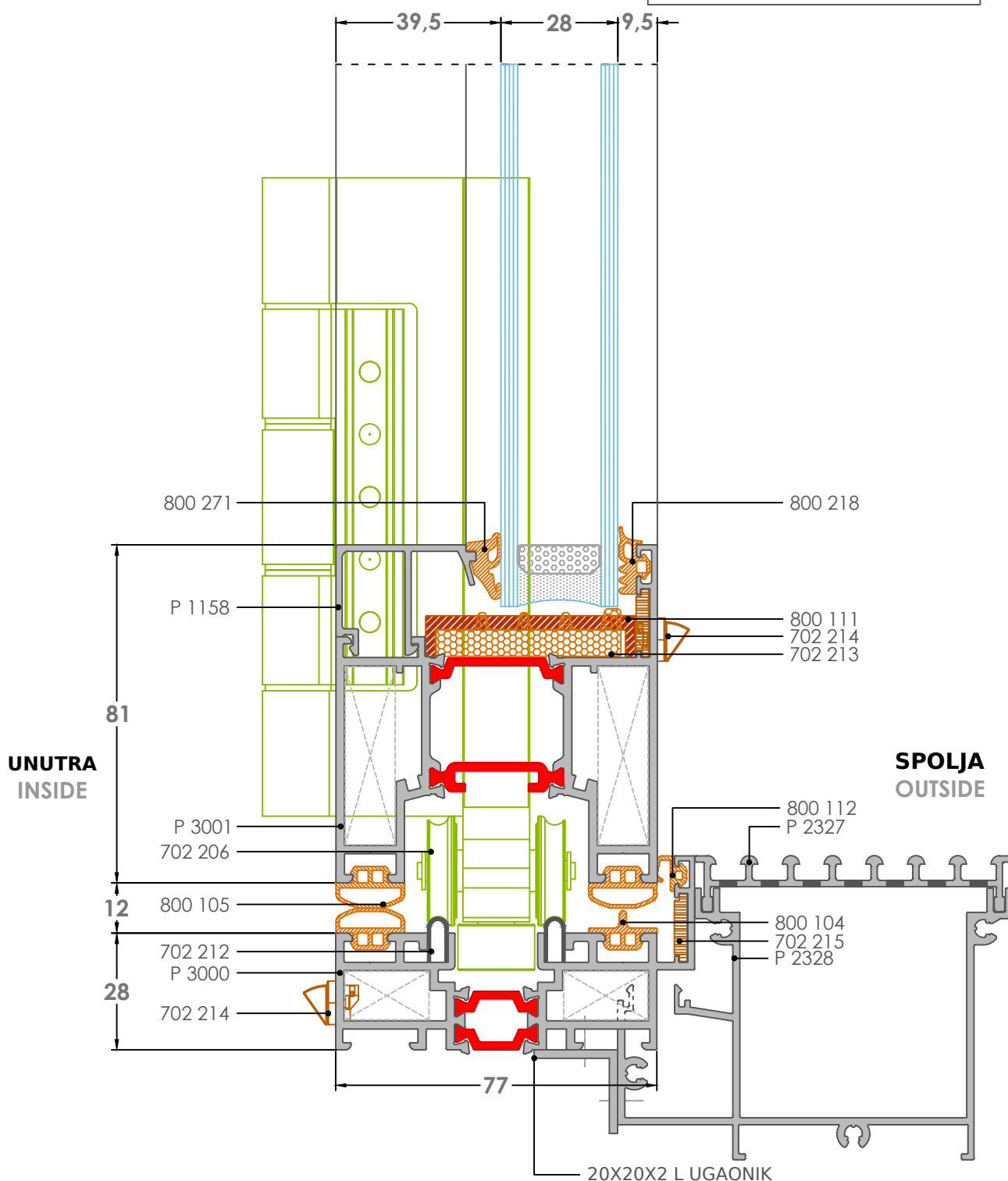
6K-3 DETALJ-Detail
