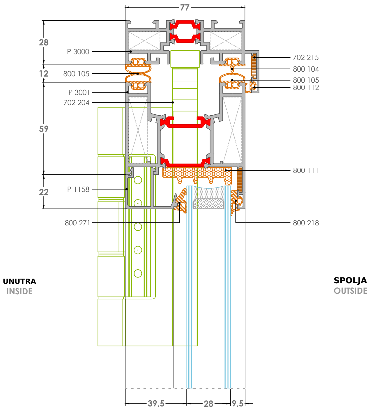
7K DETALJ-Details
