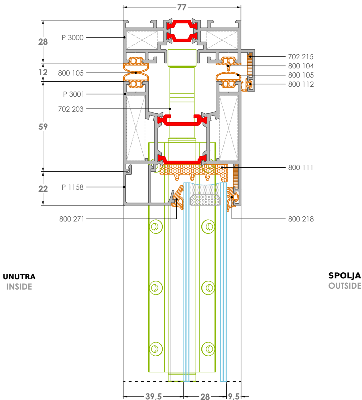
15K DETALJ-Detail
