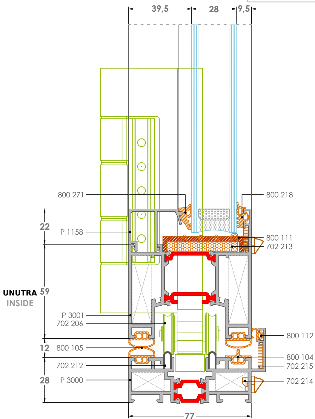
6K DETALJ-Details
