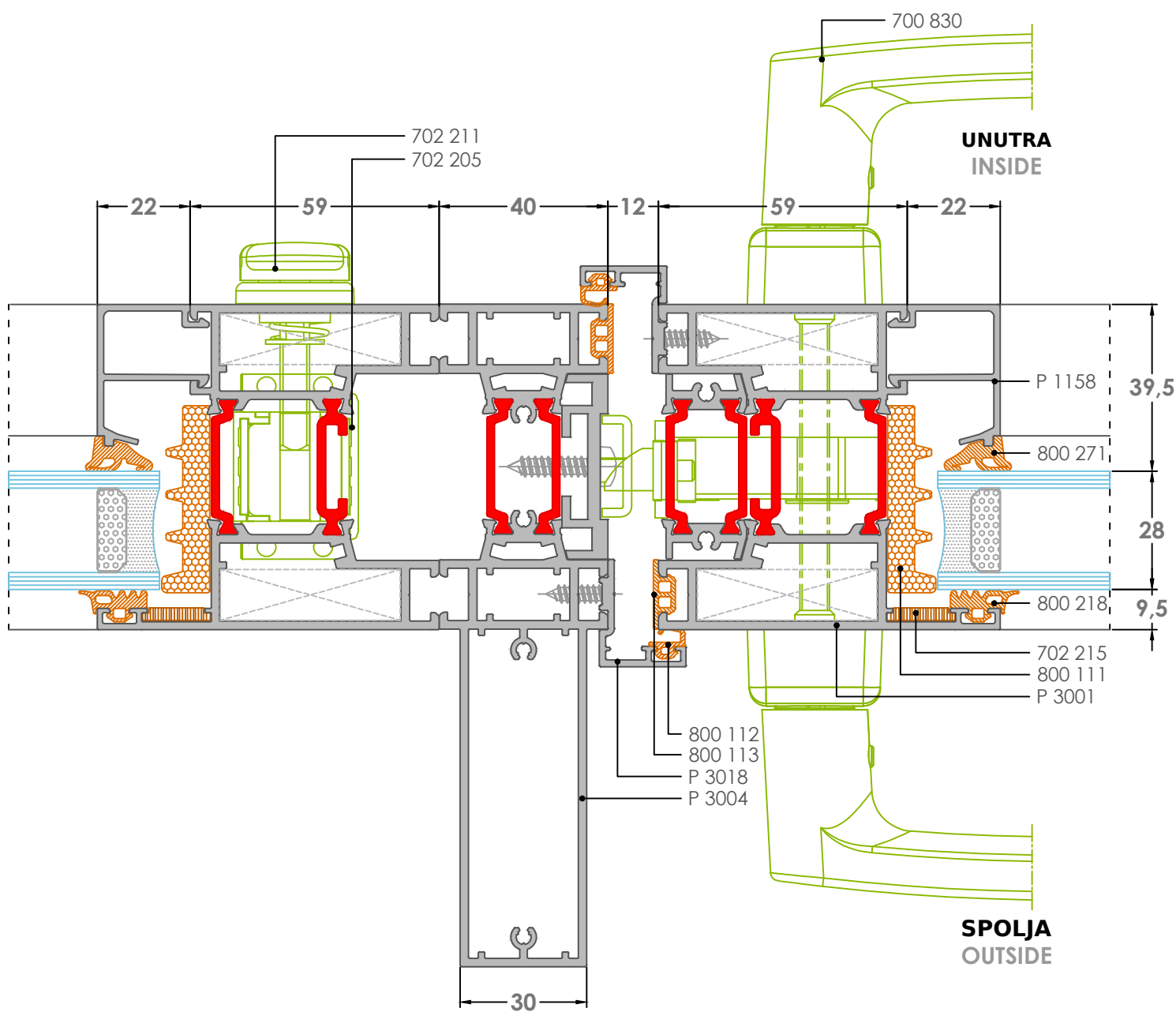
4K-5 DETALJ-Detail
