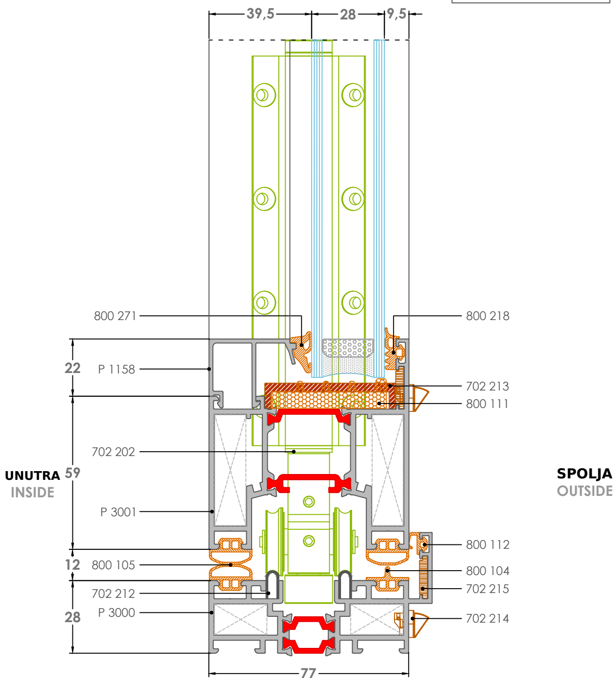
14K DETALJ-Detail
