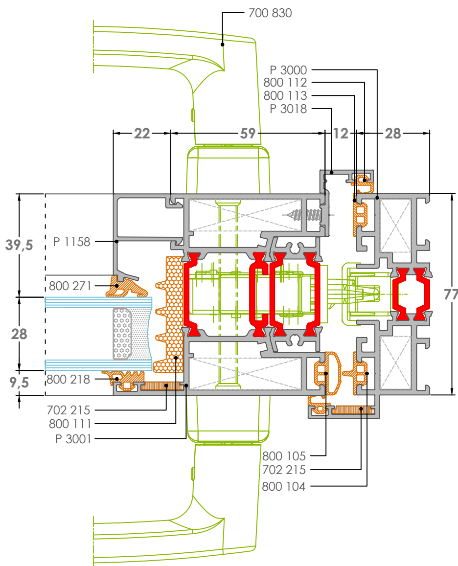
5K-2 DETALJ-Detail
