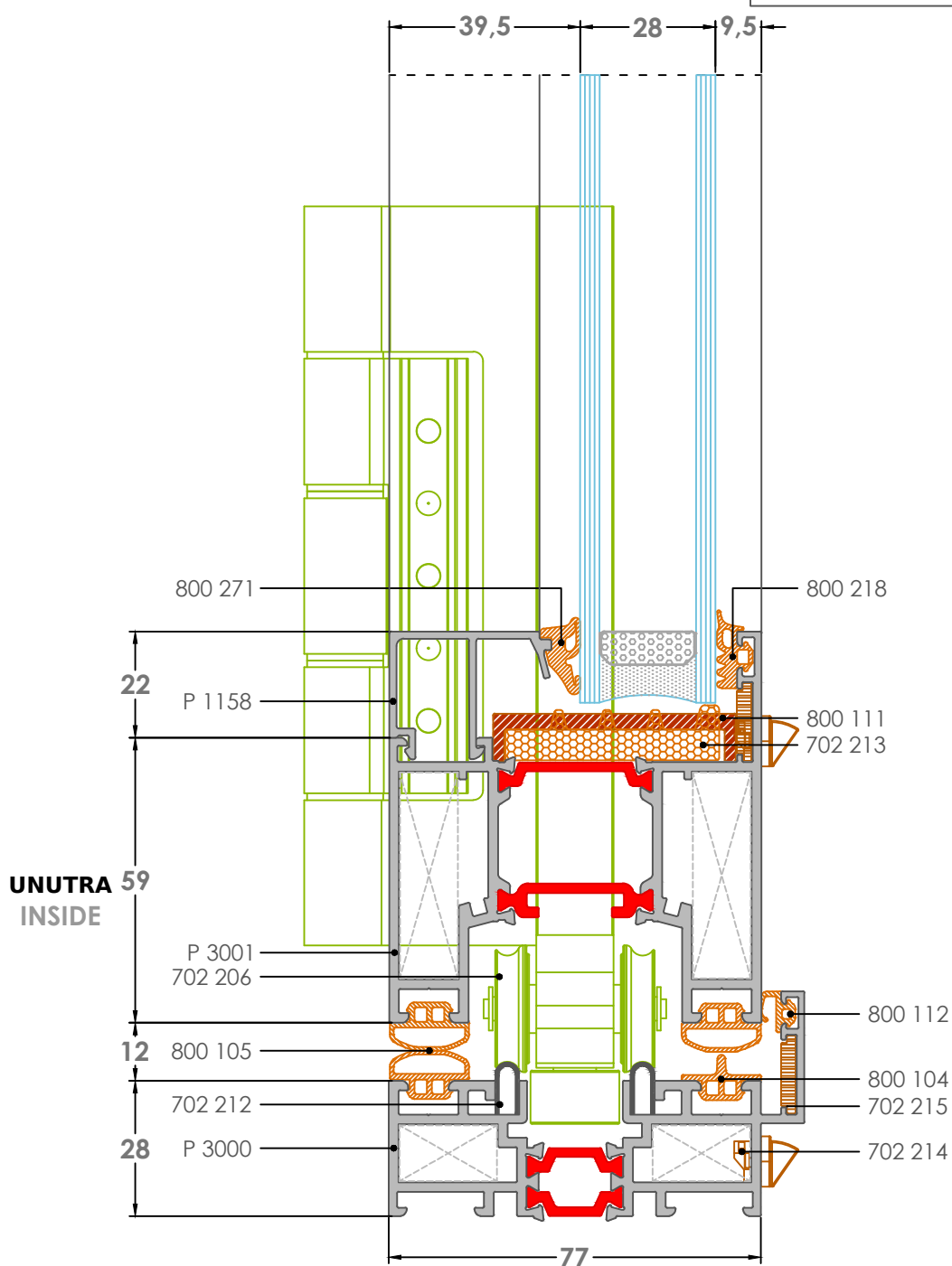
6K DETALJ-Details
