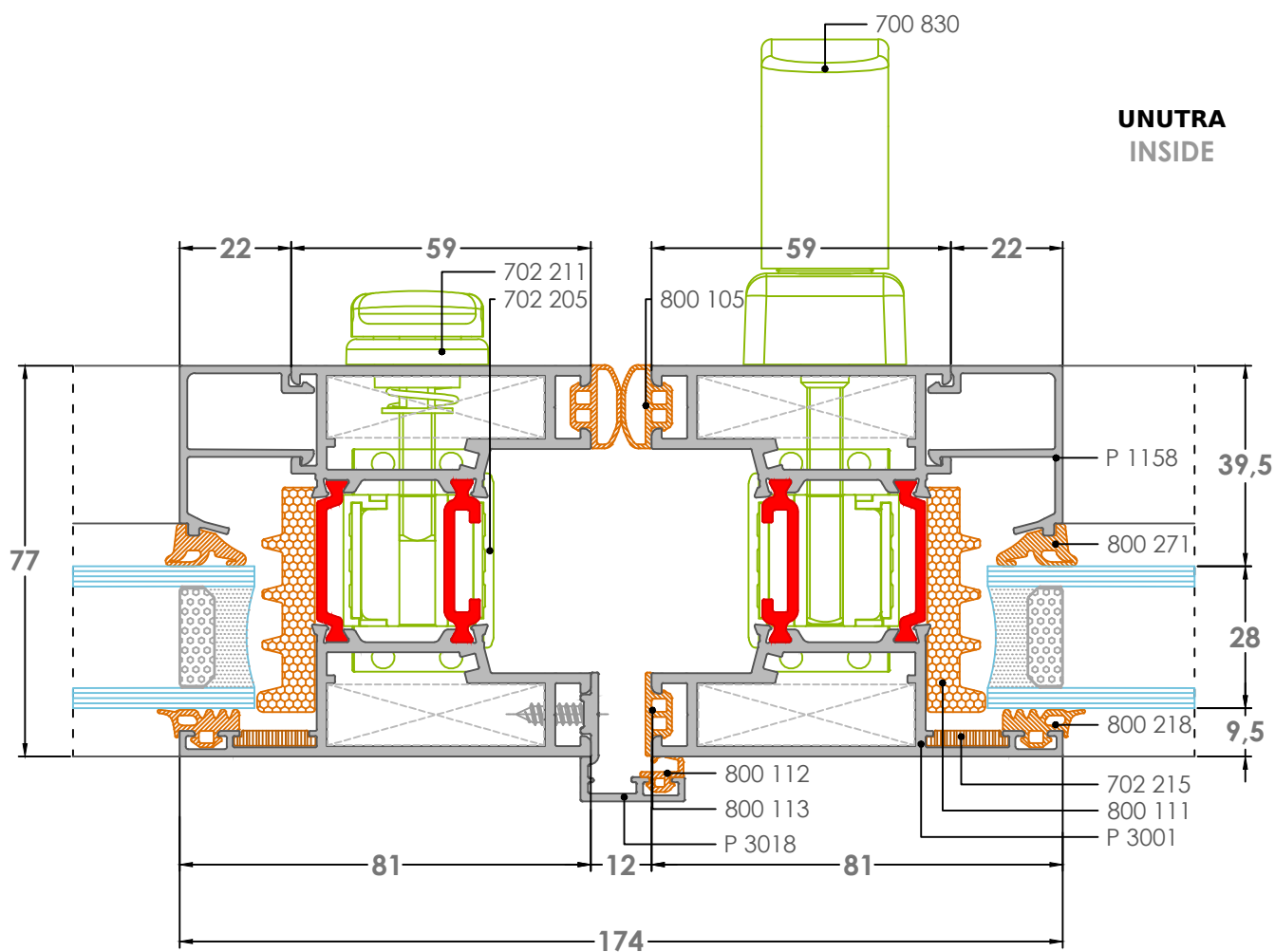
4K-1 DETALJ-Detail
