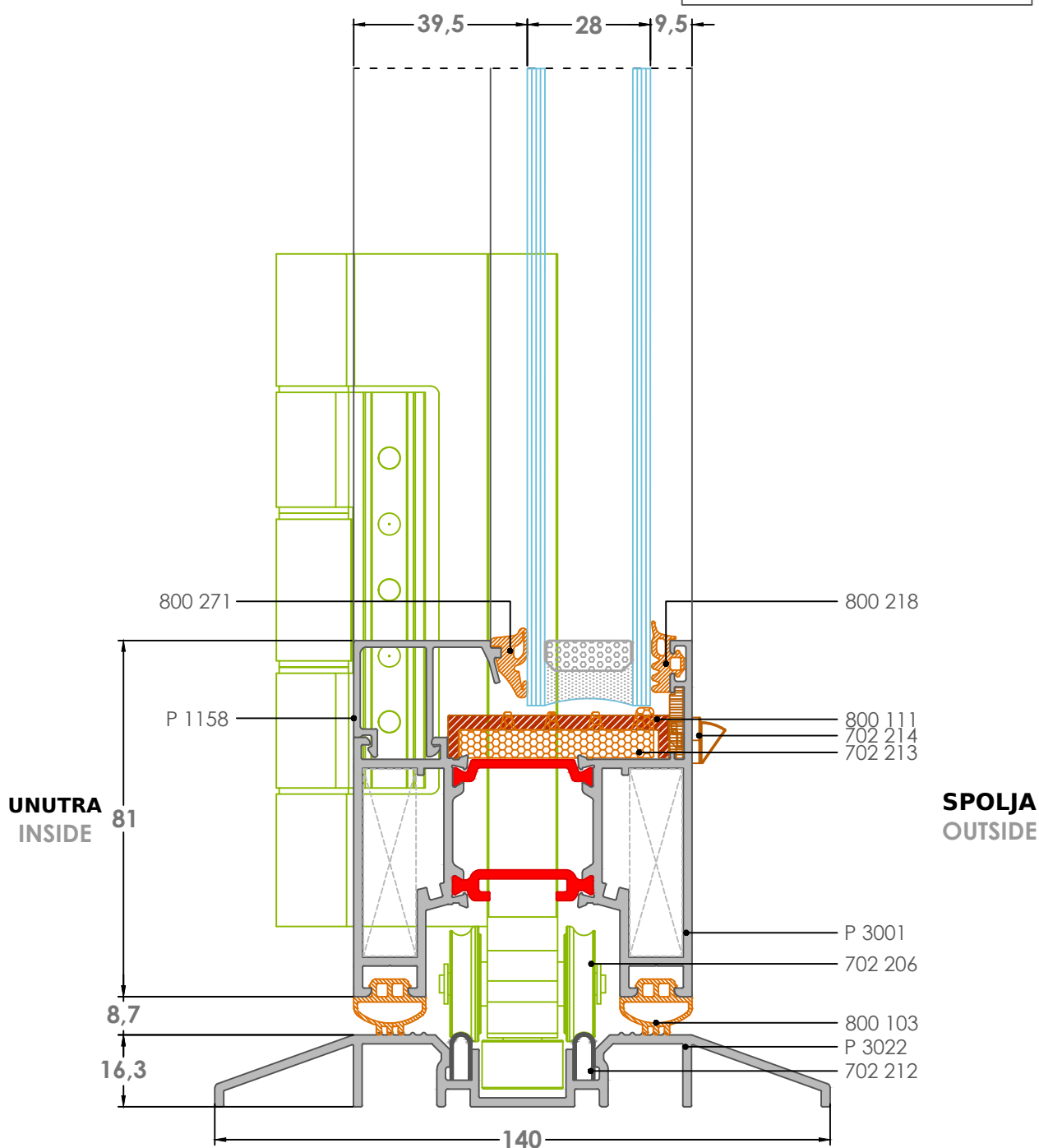
6K-1 DETALJ-Details
