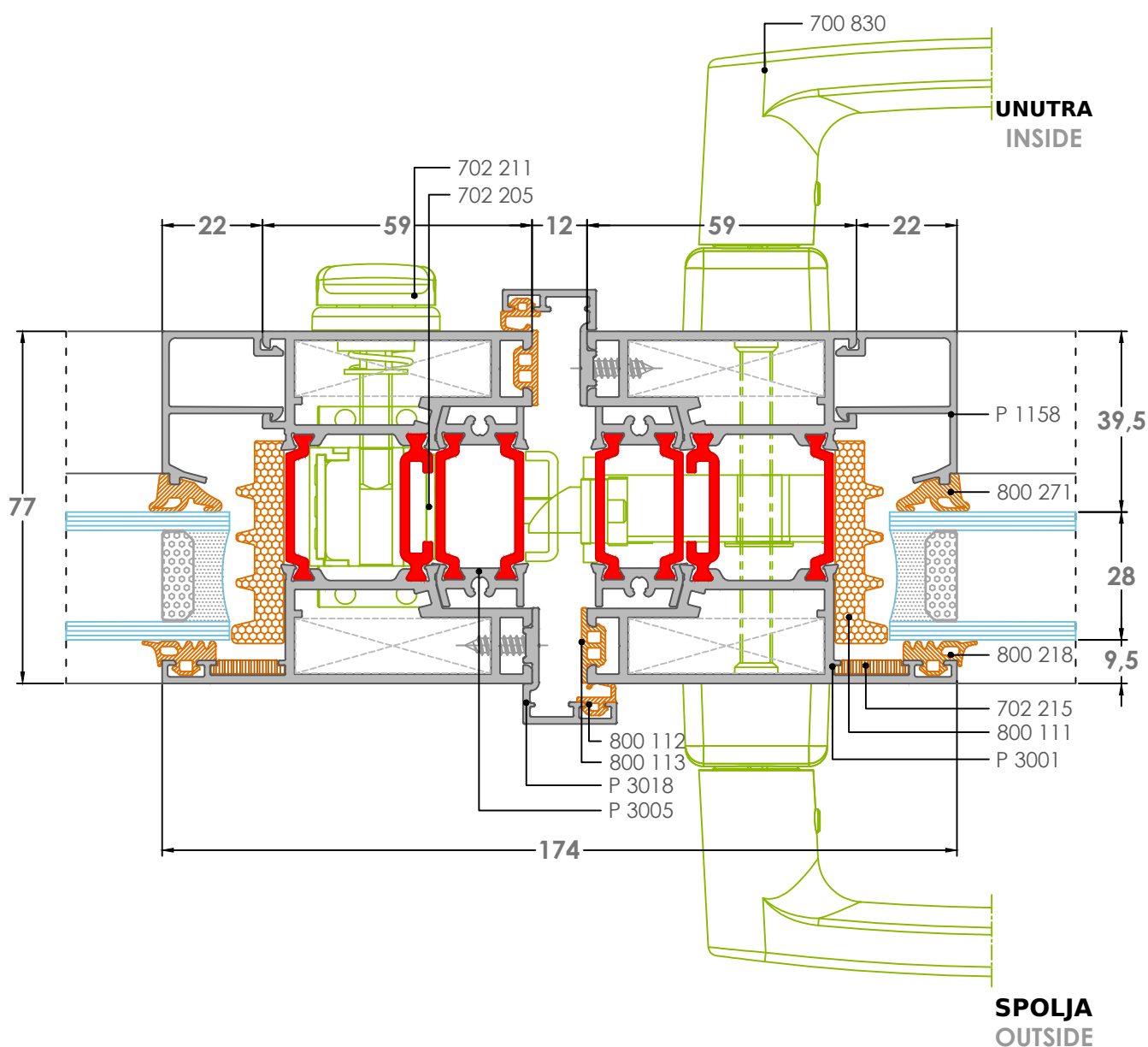
4K-3 DETALJ-Detail
