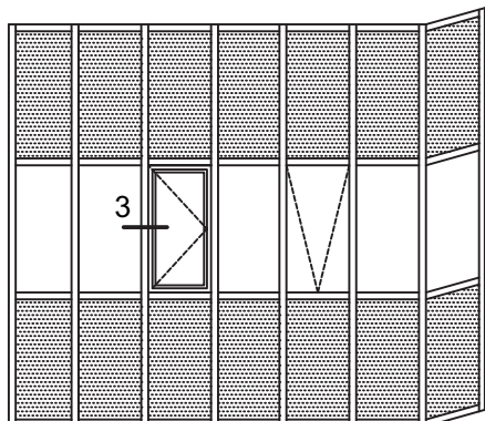
SI 66 SISTEM - VENTILACIONI OTVOR U STAKLENOJ FASADI SI 66 SYSTEM OPENING VENT IN CURTAIN WALL
