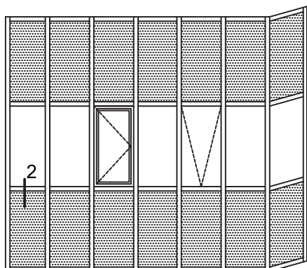
IZOLACIONI PANEL - HORIZONTALA DETALJ SPANDREL PANEL- TRANSOM DETAIL
