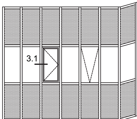
SI 58 SISTEM - VENTILACIONI OTVOR U STAKLENOJ FASADI SI 58 SYSTEM OPENING VENT IN CURTAIN WALL
