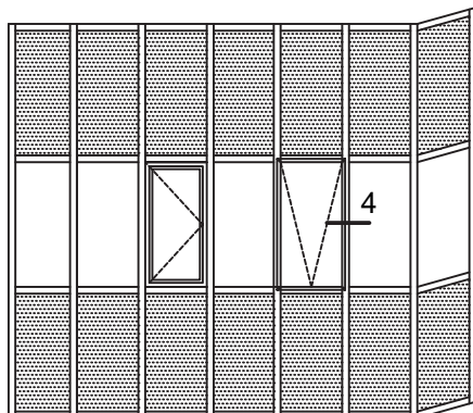
DETALJ KRILA - VERTIKALA U STAKLENOJ FASADI SASH DETAIL MULLION IN CURTAIN WALL
