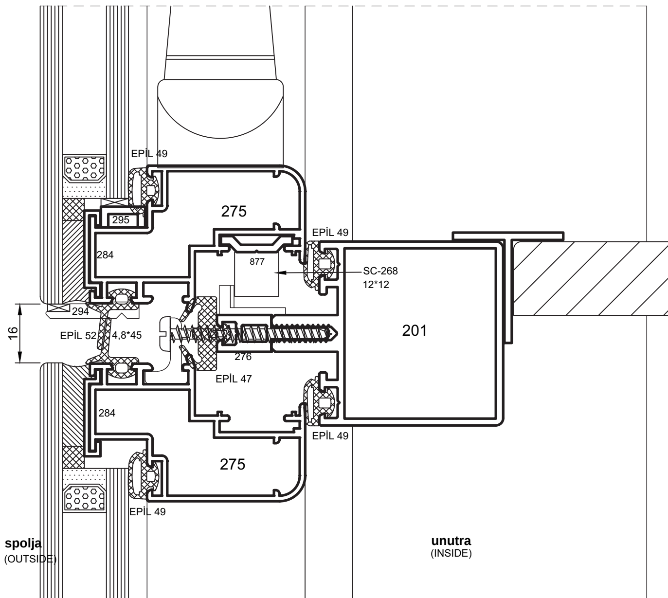
Detalj 4 Detail 4
