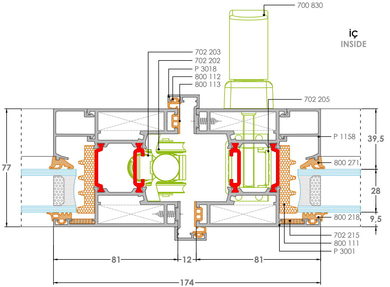
12K Detay-Detail
