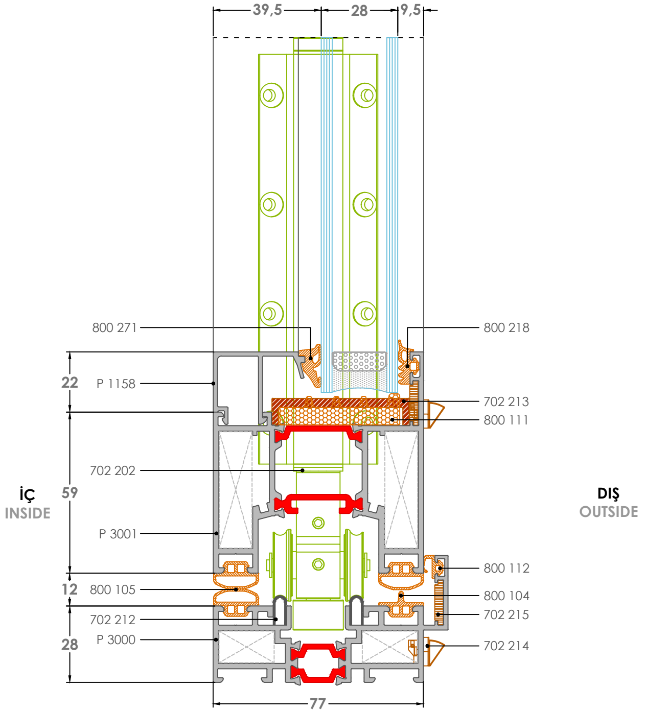
14K Detay-Detail
