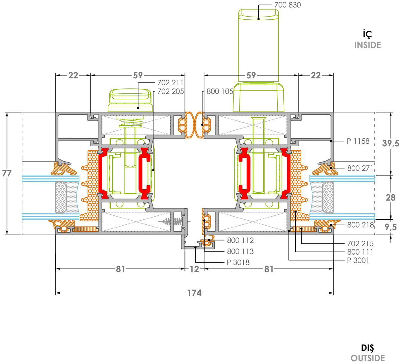
4K-1 Detay-Detail
