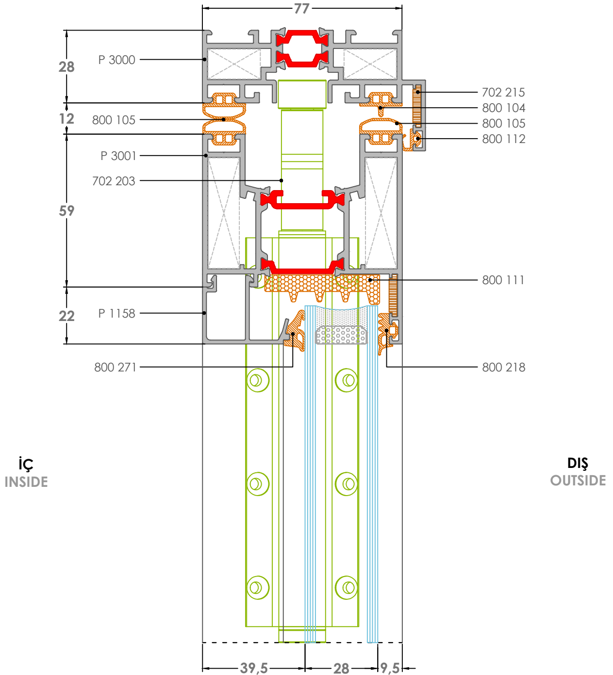
15K Detay-Detail
