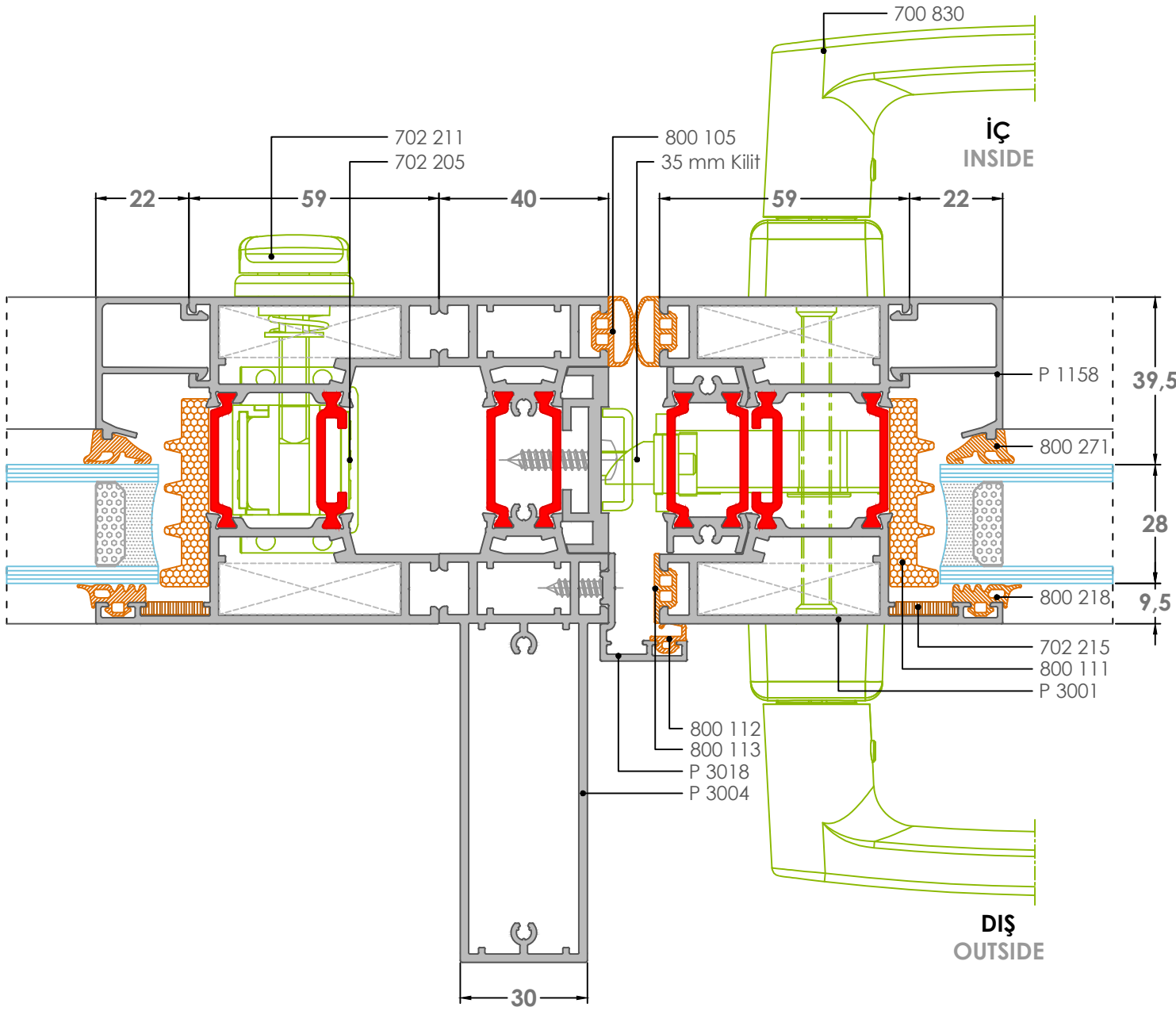
4K-4 Detay-Detail
