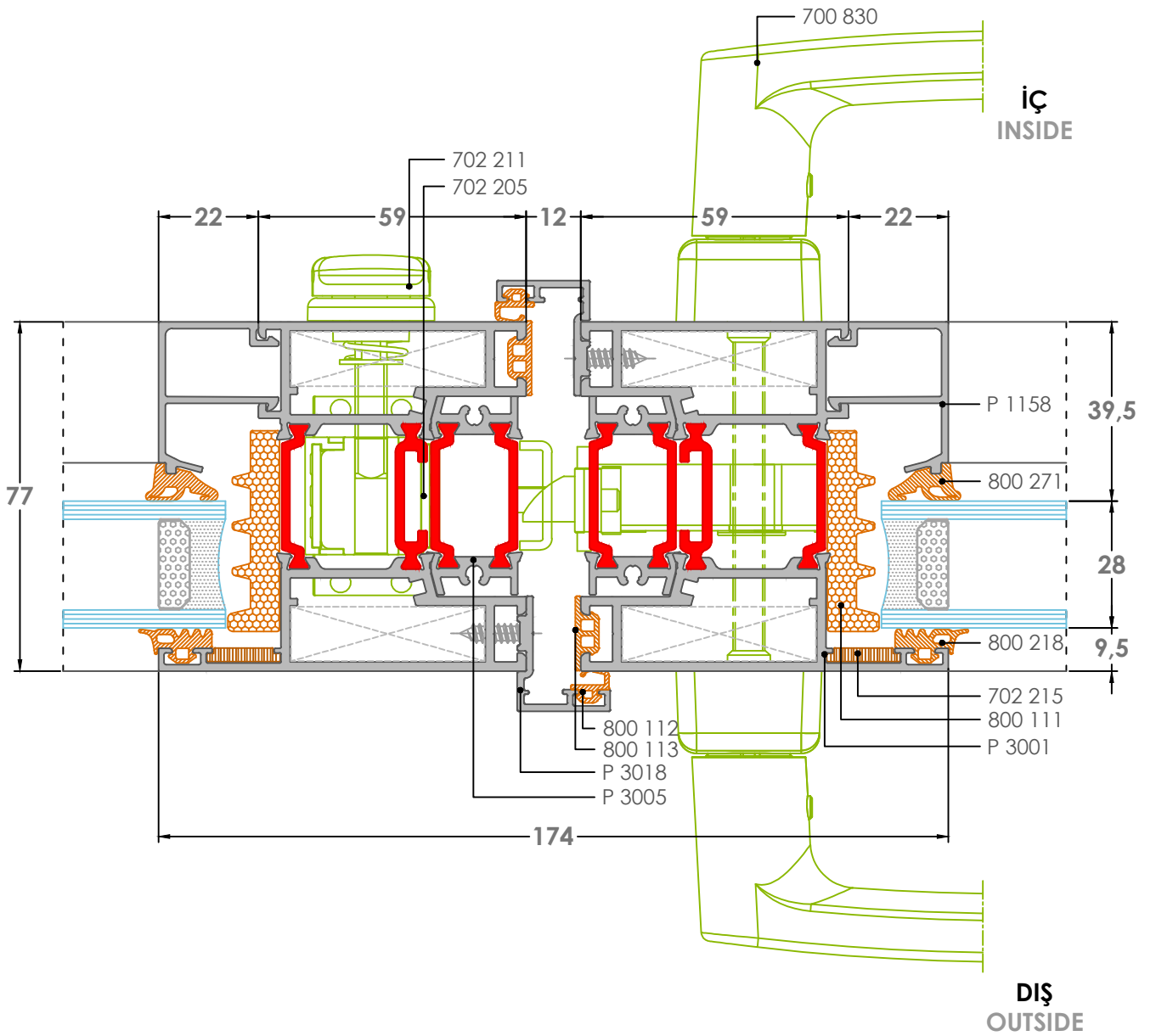
4K-3 Detay-Detail
