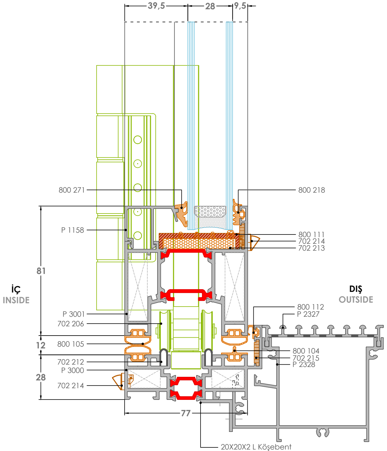
6K-3 Detay-Detail
