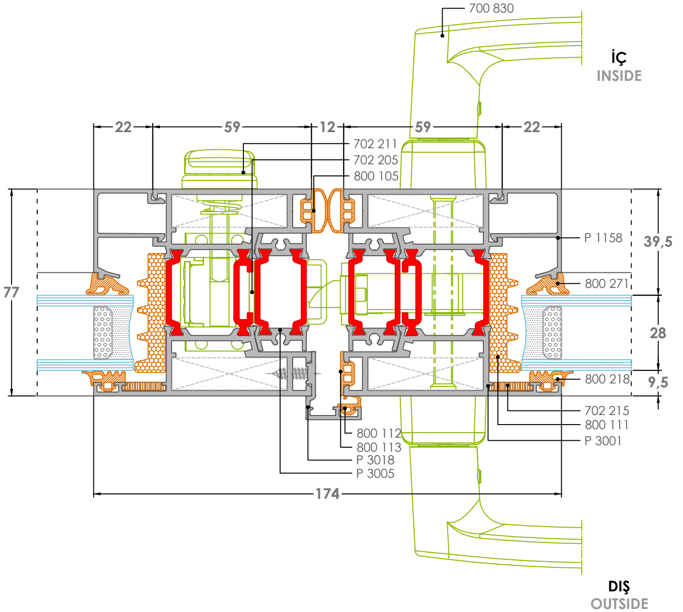
4K-2 Detay-Detail
