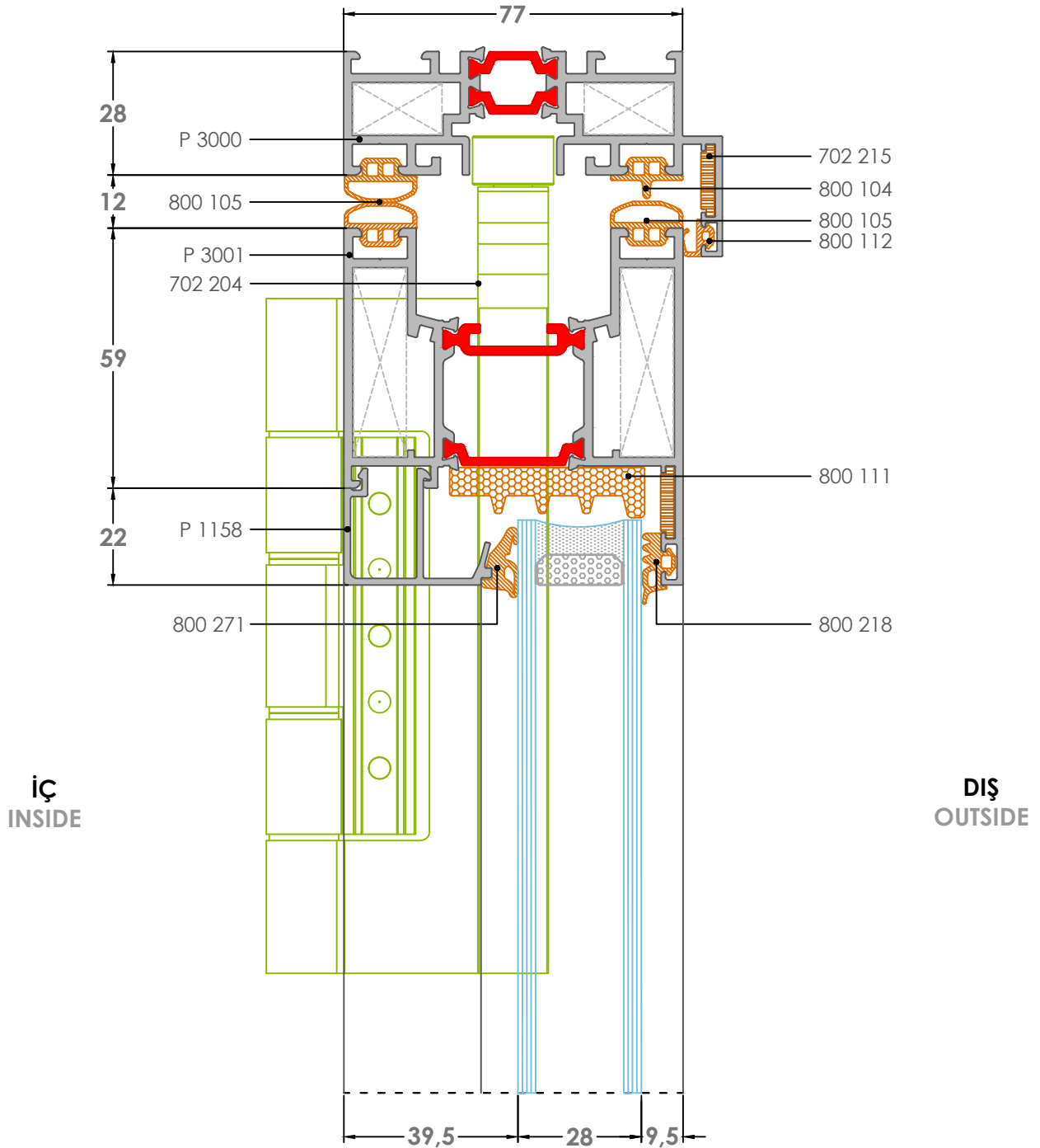
7K Detay-Detail
