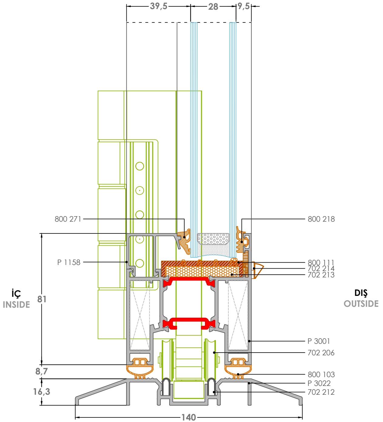
6K-1 Detay-Detail
