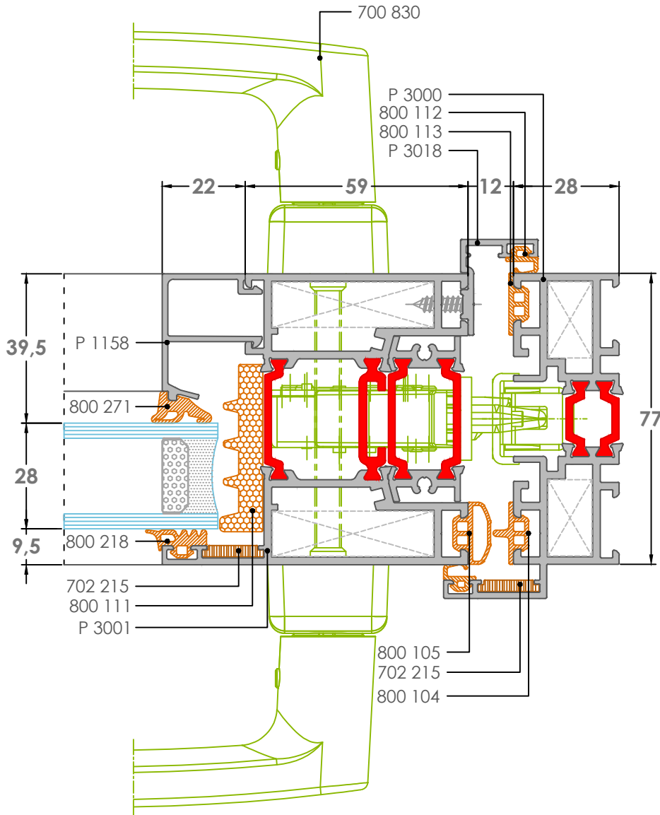
5K-2 Detay-Detail
