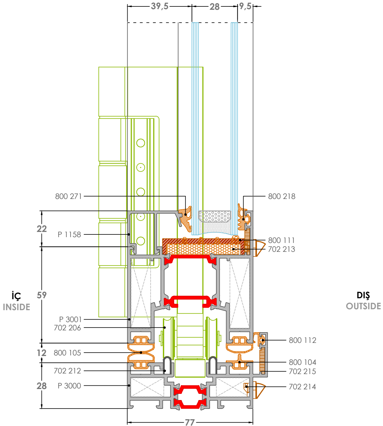
6K Detay-Detail
