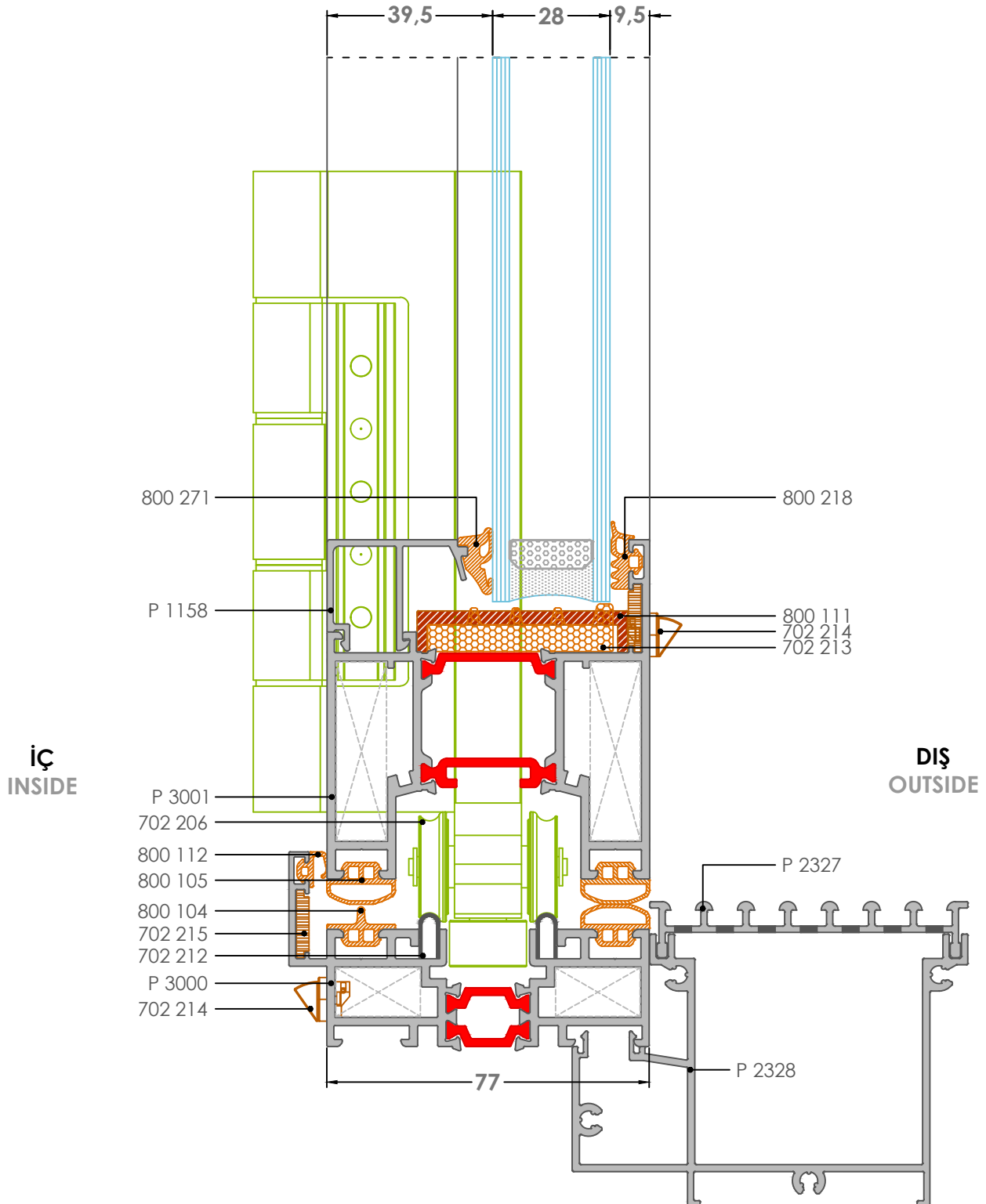
6K-2 Detay-Detail
