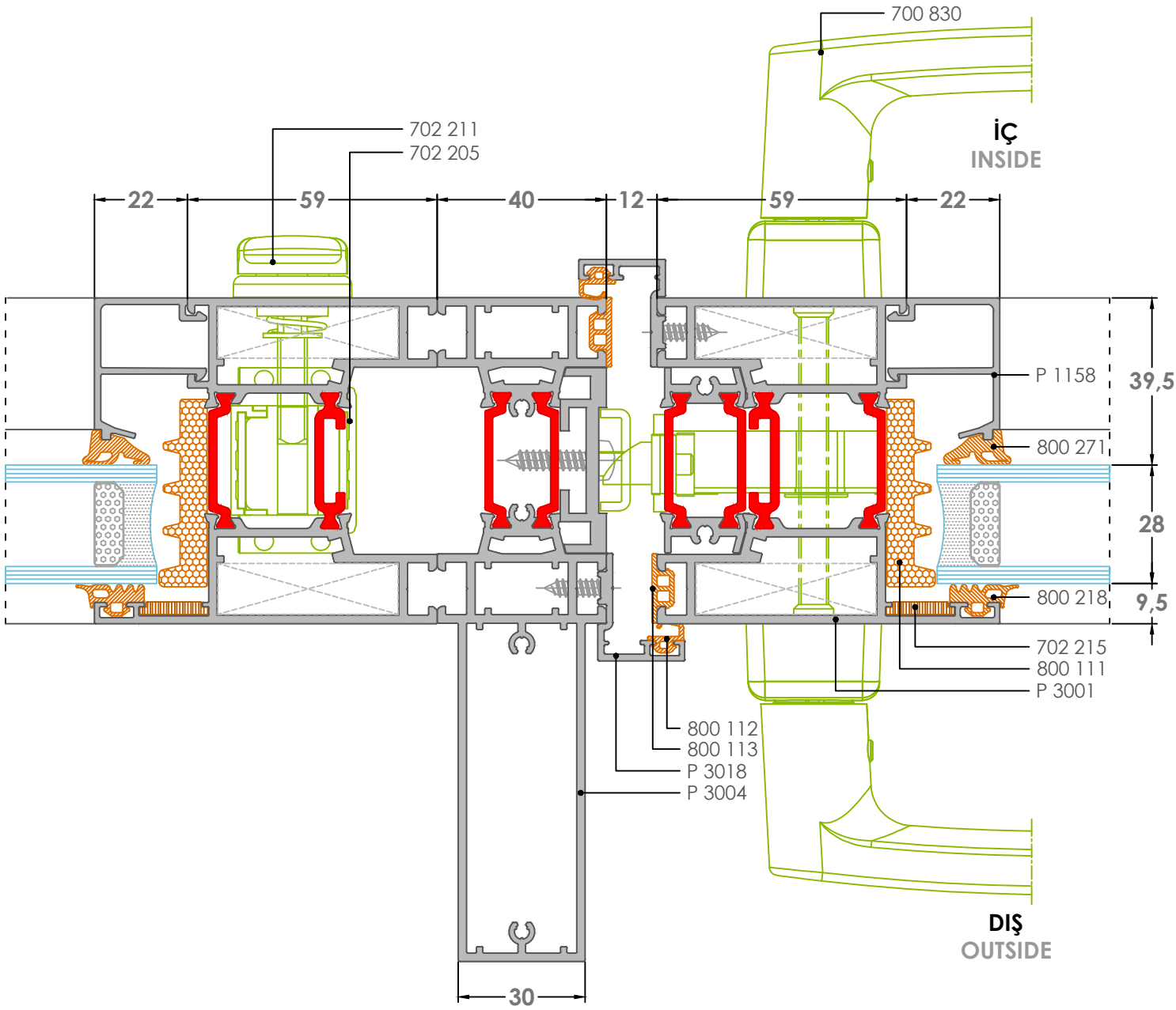
4K-5 Detay-Detail
